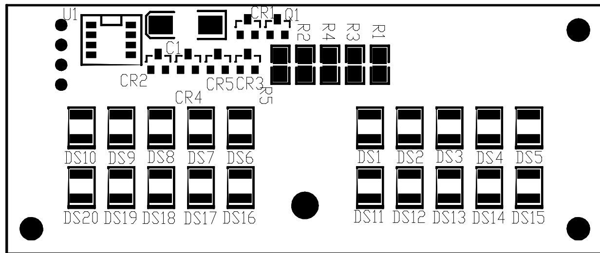
PRIMARY SIDE
