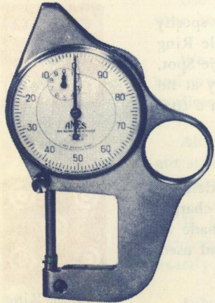
No. A-3. Perfection Dial Micrometer . . . Each $35.00
