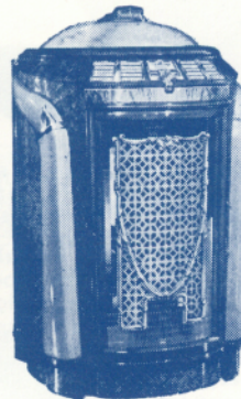
SEEBURG 148-147-146 20 records/ 20 selections/78 rpm H. 57" W. 36" D. 26 \frac{1}{2} " Net. Wt. 355 lbs. Ship. Wt. 450 lbs.
