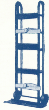
Sled-Type Appliance Carrier Model 7706 Carrier 6" deep, 16" wide. 57 1/2" high frame. Two wide holding belts. 5" x 23" solid steel nose plate. Solid rubber wheels 2" wide, 6". Load capacity up to 750 pounds. — $32.50 —
